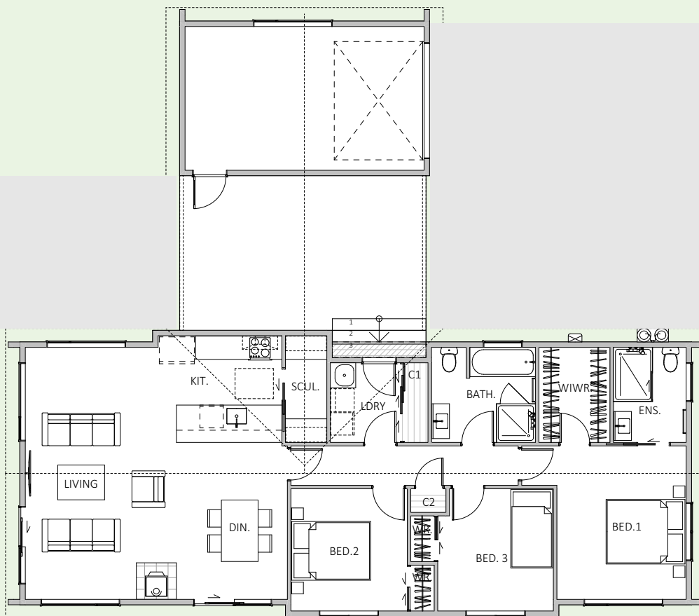
floorplan is shown with carport and single garage, which is an additional cost
