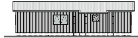
Elevation C
